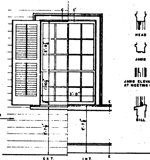
TYPICAL WINDOW AND WINDOW SECTION
