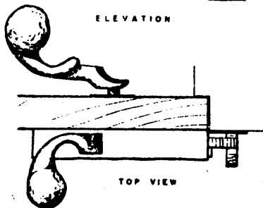
WROUGHT IRON BOX LOCK AND KEEPER SCALE 6"=1'-0"
