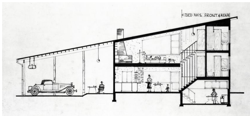
Sketch of Kohler residence from the Harris Armstrong Collection, Washington University Archives, courtesy of Andrew Raimist.
