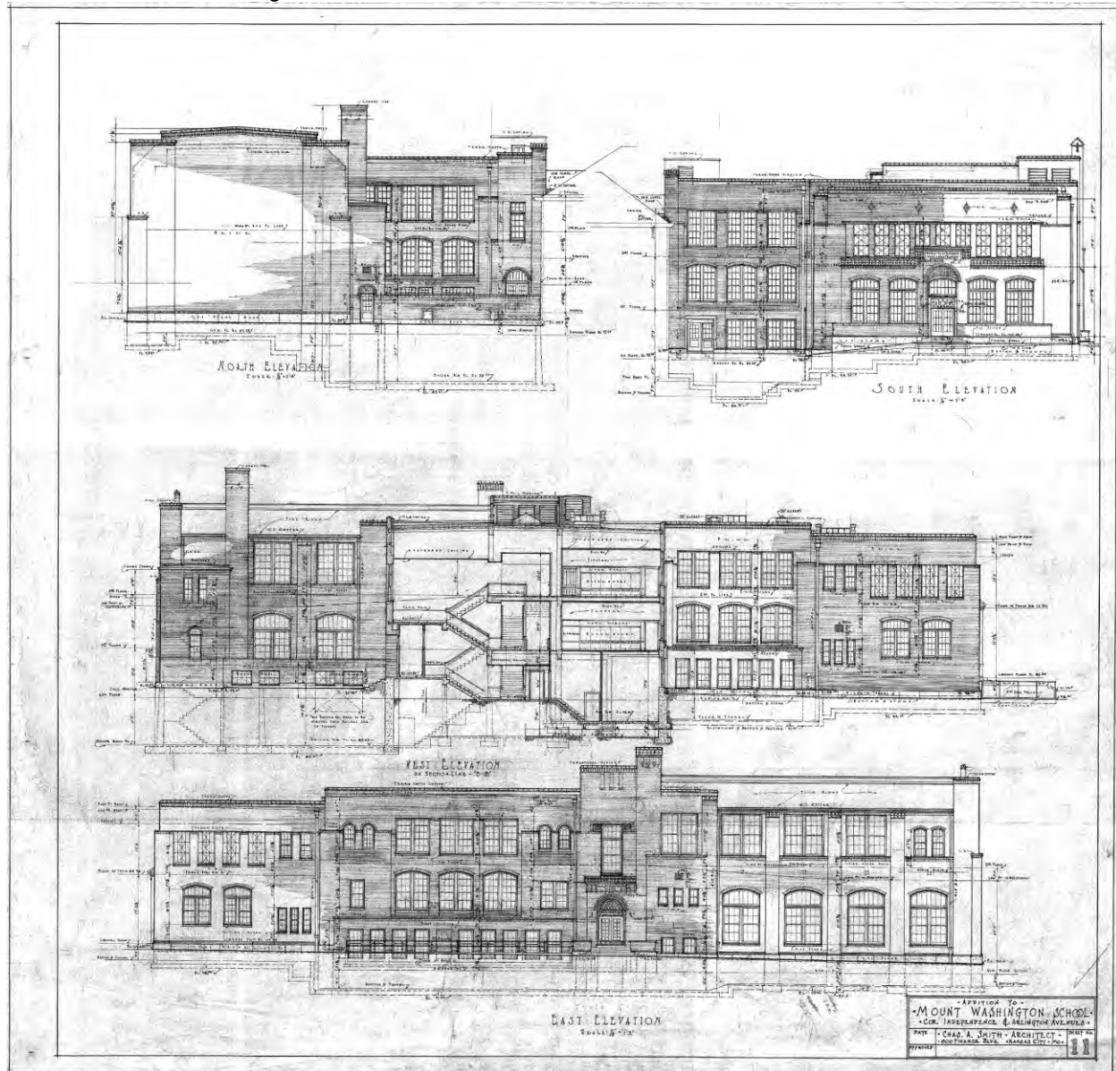
Figure 4. Elevations, Historic Plans, Charles A. Smith, 1924.
