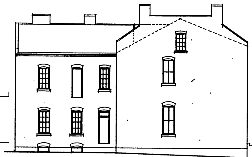
EAST ELEVATION SCALE 1/4" = 1'-0"
