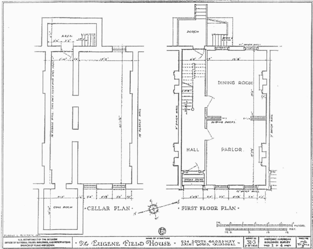
Figure 1. Eugene Field House Floor Plans – Cellar and First Floor Historic American Buildings Survey, 1934
