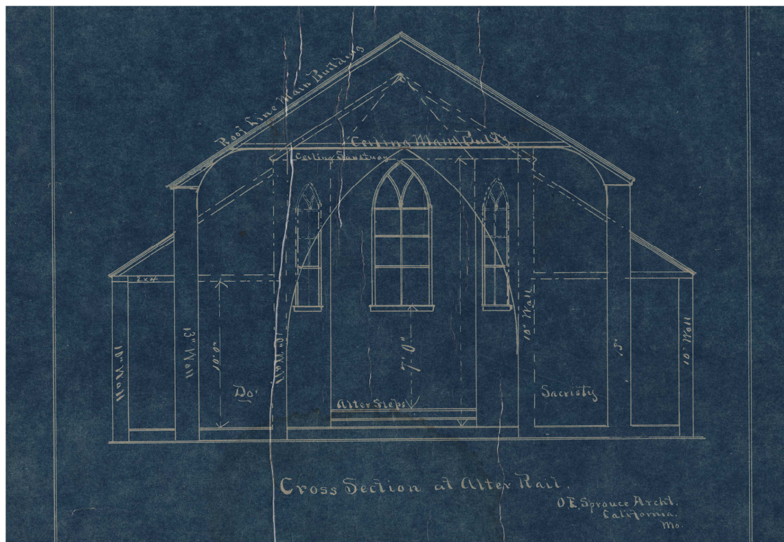
Figure 5: Cross Section at altar rail, O.E. Sprouce, 1903.
